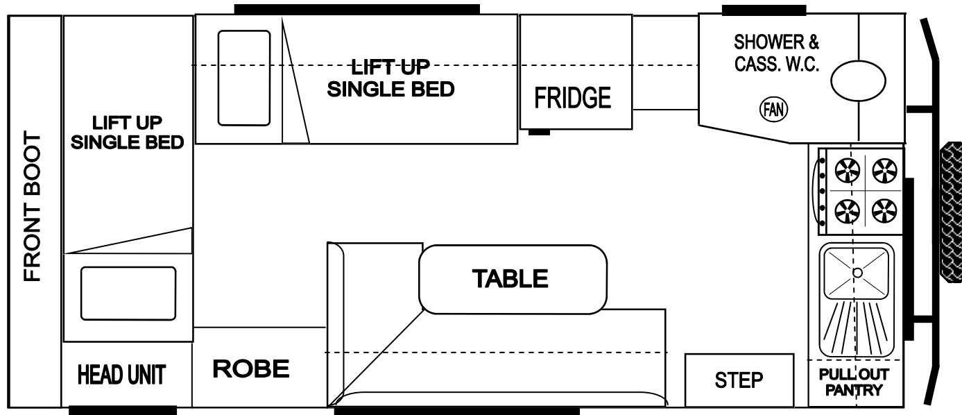
NULLARBOR 16' X 7' 6" (4.9m x 2.3m)
