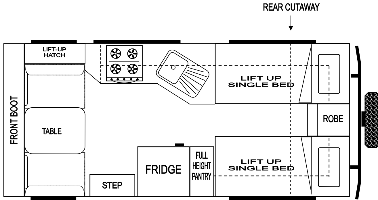
KIMBERLEY 15' x 7' (4.6m x 2.3m) CROSS COUNTRY
