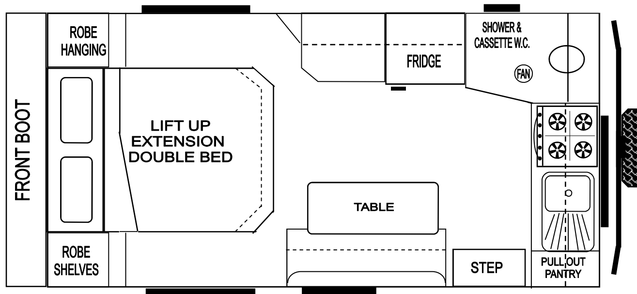
KIMBERLEY 15' x 7'6" (4.6m x 2.3m)
