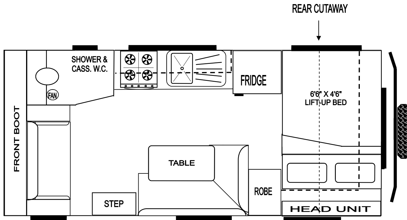
NULLARBOR 16' X 7'6" (4.9m x 2.3m) CROSS COUNTRY
